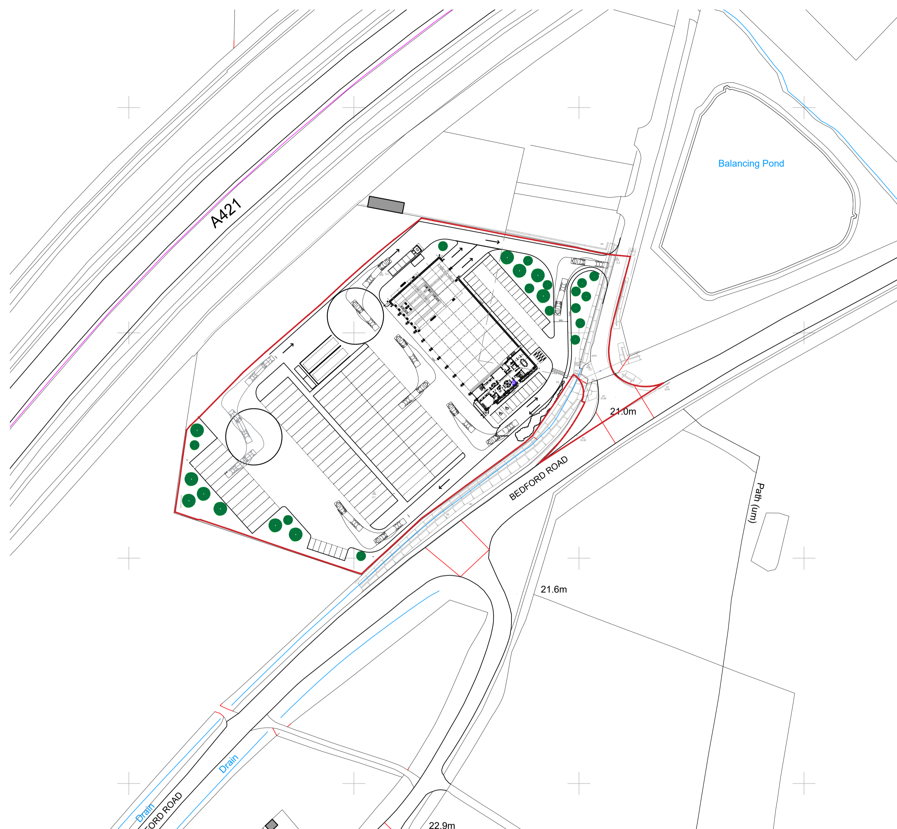
SITE/BLOCK PLAN - 1:1000
