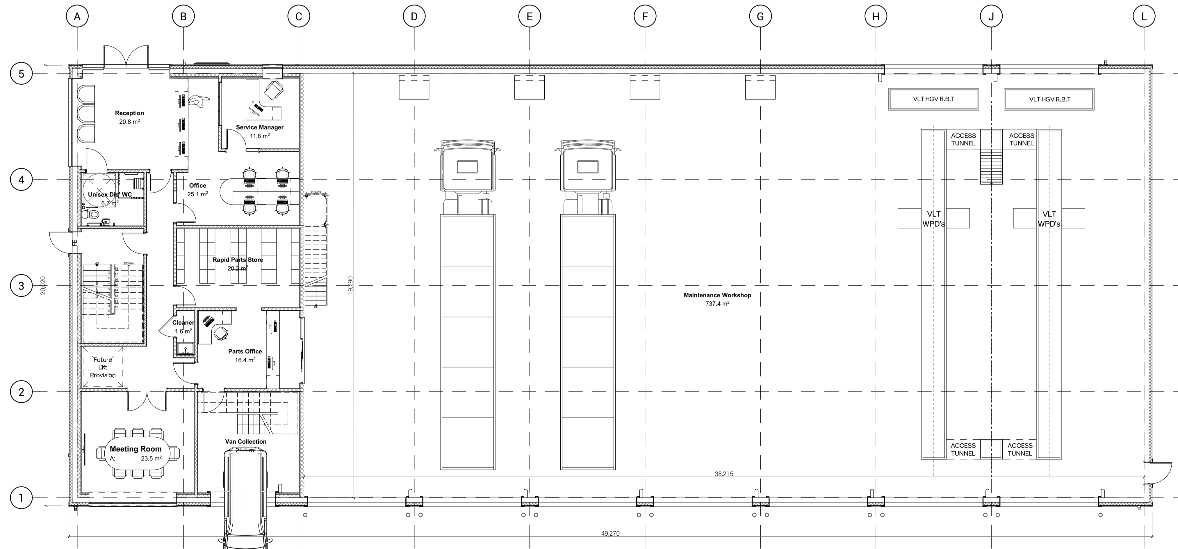
GROUND FLOOR AS PROPOSED
