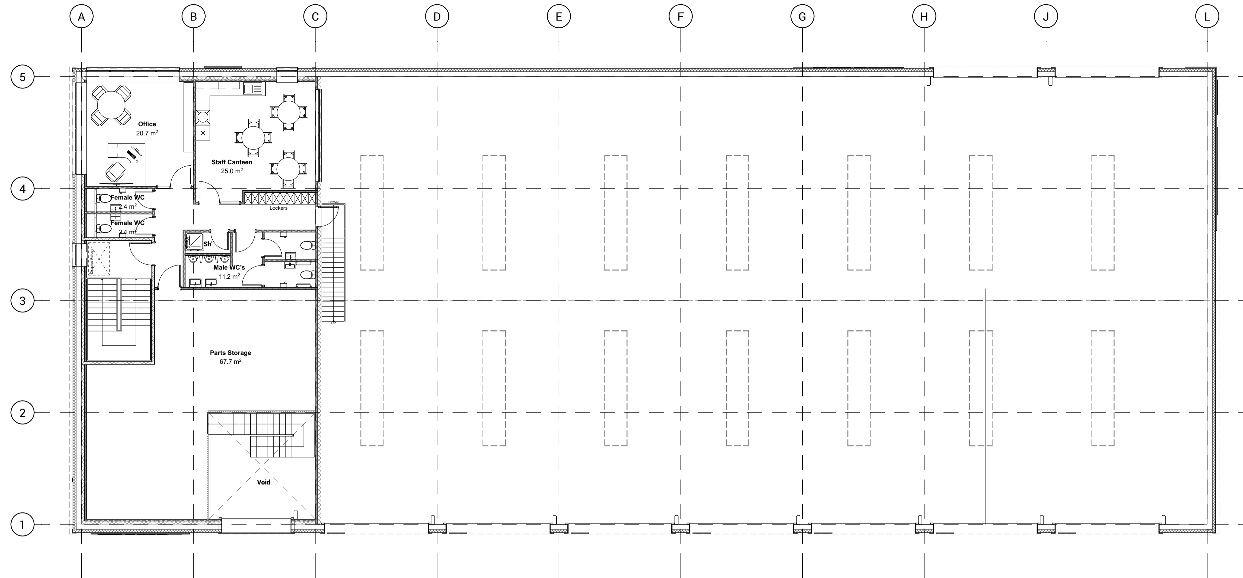
FIRST FLOOR AS PROPOSED
